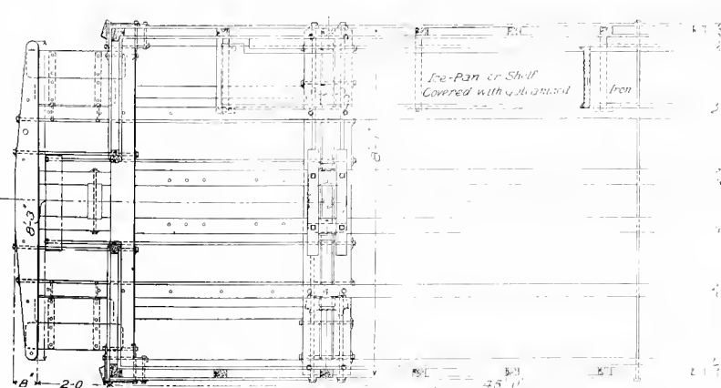
Fig. 273b. Part Plan Showing Underframe.
